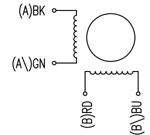
WIRING DIAGRAM
